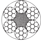
6 x 7 (1+6) + FE
