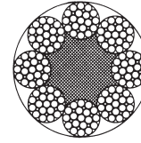
8 x 19 Filler (1+6+6F+12) + FE
