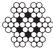
6 x 7 (1+6) + SEL
