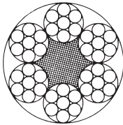
6 x 7 (1+6) + FE
